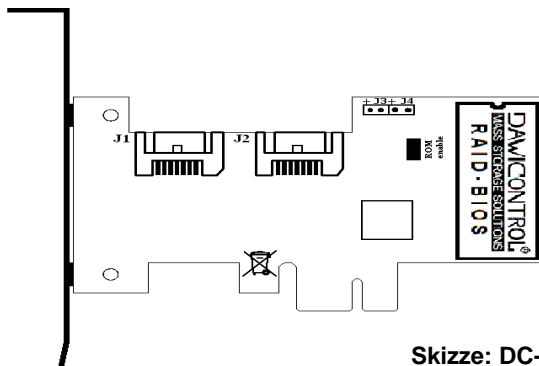
Skizze: DC-300e RAID
