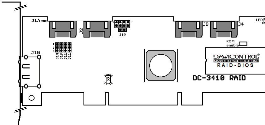
Skizze: DC-3410 RAID
